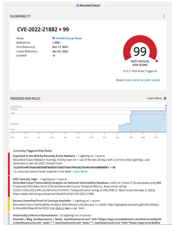
Example vulnerability Intelligence Card showing comprehensive intelligence including risk score, risk rules, transparency to original sources of intelligence, and more
