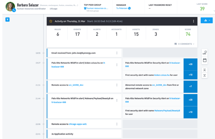
Figure 2. Exabeam Smart Timeline showing how a malicious email caused a malware payload drop.
